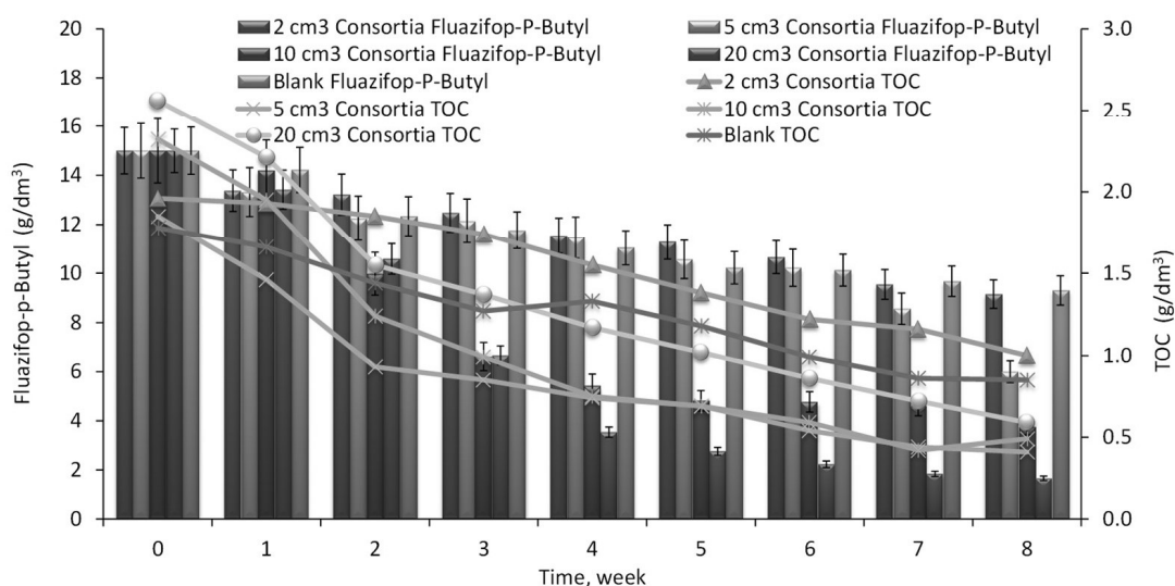
Fig. 4. Time dependences of fluazifop-p-butyl content and TOC for various contents of the homogenised bacterial mixture (2–20 cm 3 ) in the sterile agricultural soil
