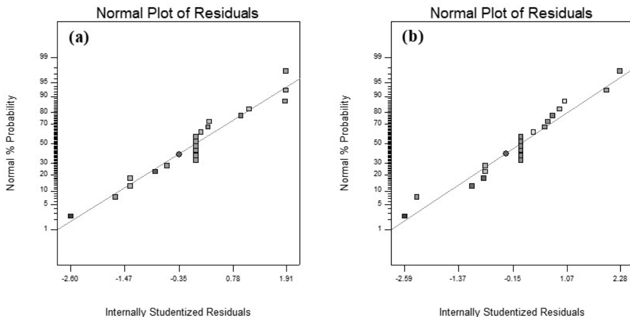
Fig. 3. Normal probability plots of residual for RBV 5R removal (%) (a) and BG removal (%) (b).
