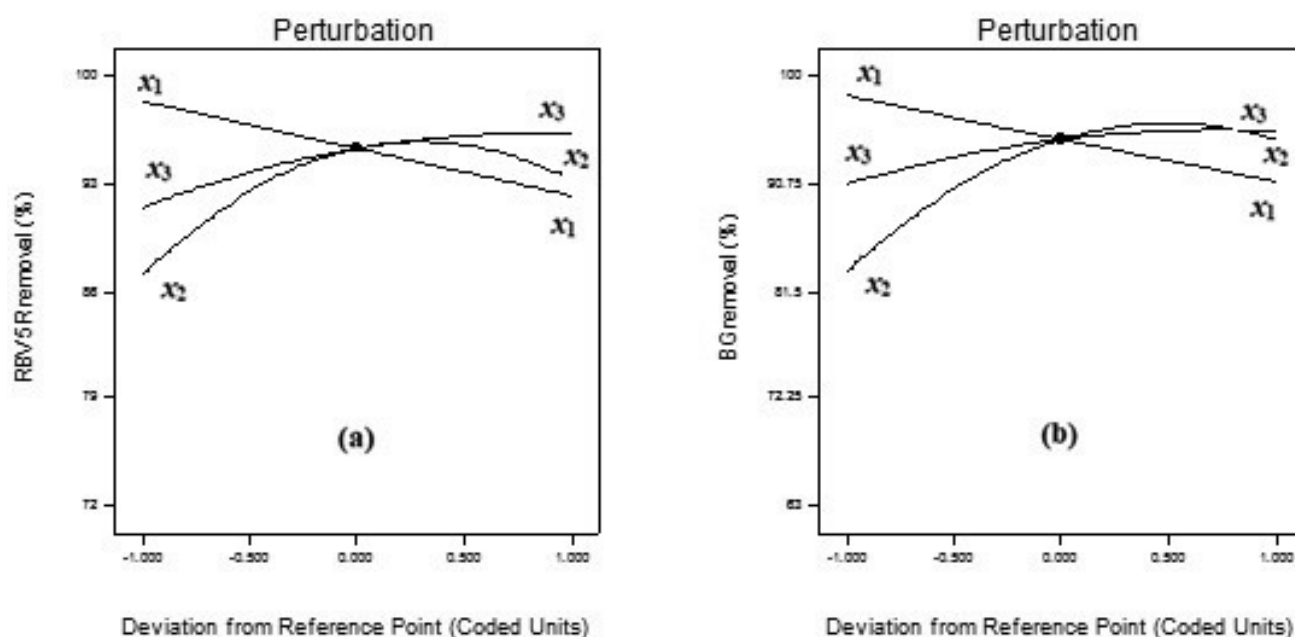
Fig. 4. Perturbation plots for RBV 5R (a) and BG (b) removal.
