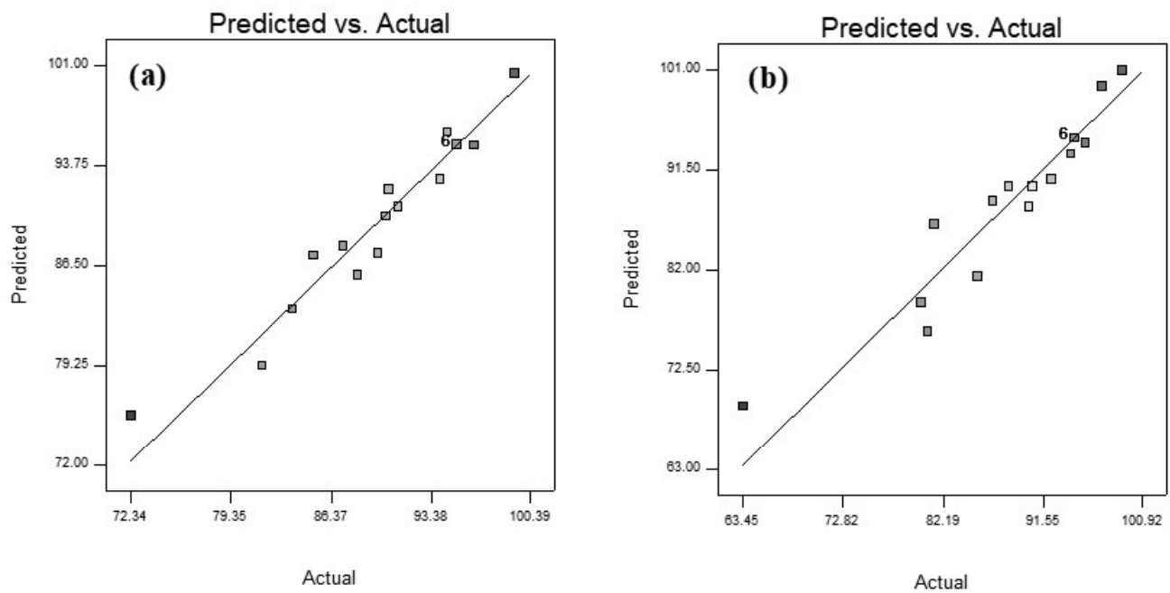
Fig. 2. Comparison plot between the experimental and model predicted RBV 5R removal (%) (a) and BG removal (%) (b).
